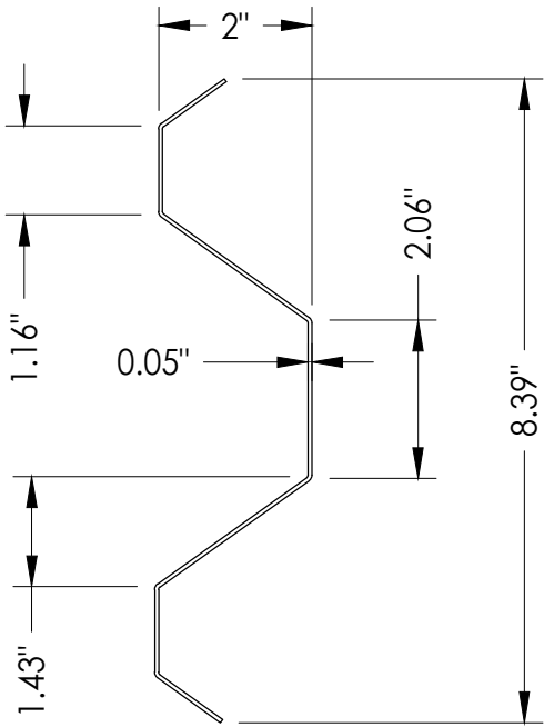
4 EXTERIOR CORRUGATED PANEL 1/2 SCALE
