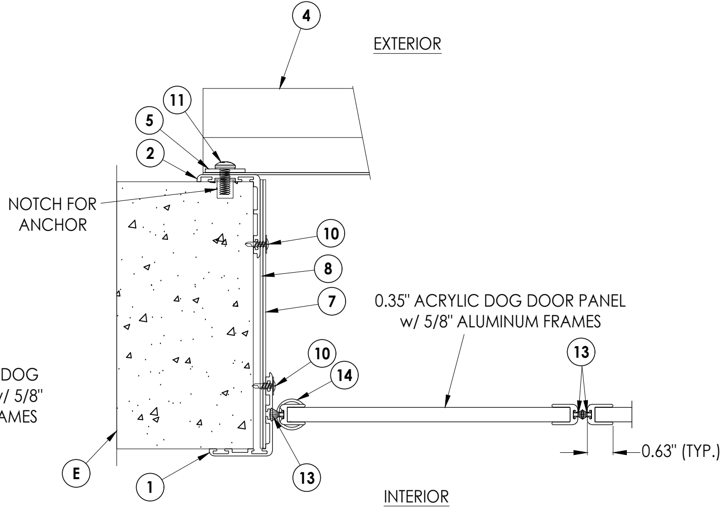
2 4 HORIZONTAL CROSS SECTION FOR PLEXIDOR SIZES LGP & XL (UP TO 20.375" X 26.625")
