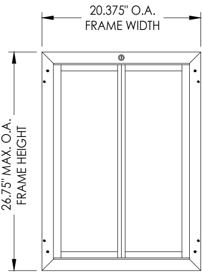
INTERIOR VIEW PD HURCAN WALL MOUNT (X-LARGE)
