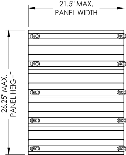
EXTERIOR VIEW w/ CORRUGATED PANELS
