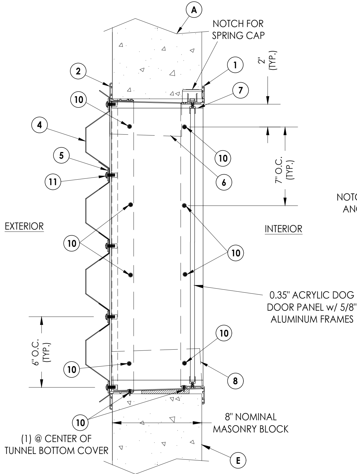
1 4 VERTICAL CROSS SECTION Shown w/ X-Large Size Dog Door Masonry Framing Installation
